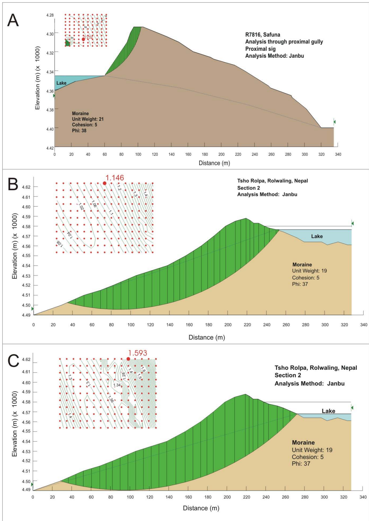
Fig. A3.1: Example outputs from Slope/W slope stability modelling software: (A) application to moraine stability assessment, Laguna Safuna, Peru; (B) and (C) to determine level of lake drawdown required to achieve satisfactory factor of safety, Tsho Rolpa, Nepal.
