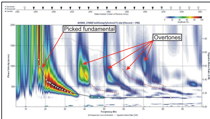
Figure 2: A dispersion image displayed in SurfSeis software (Kansas Geological Survey). Pre-processing to improve data interpretability has been carried out. The fundamental mode has been picked manually. Multiple overtones are also clearly identifiable.
