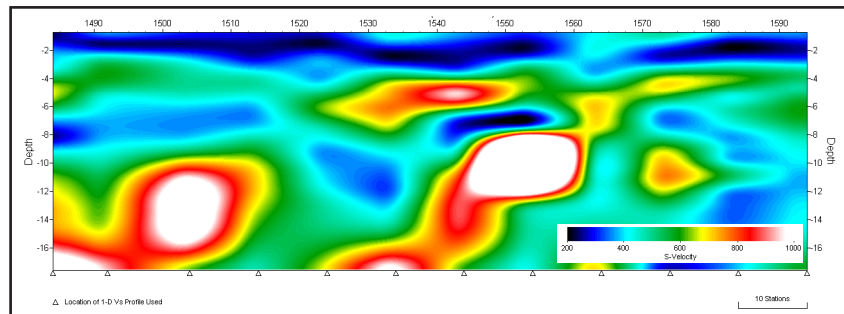
Figure 3: A 1.5D V_s section displayed in SurfSeis software. Component 1D sections were produced by gradient-based, iterative inversion of manually picked fundamental dispersion curves.
