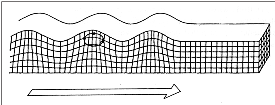
Figure 1: Rayleigh wave particle motion (from Bolt, 1982).
