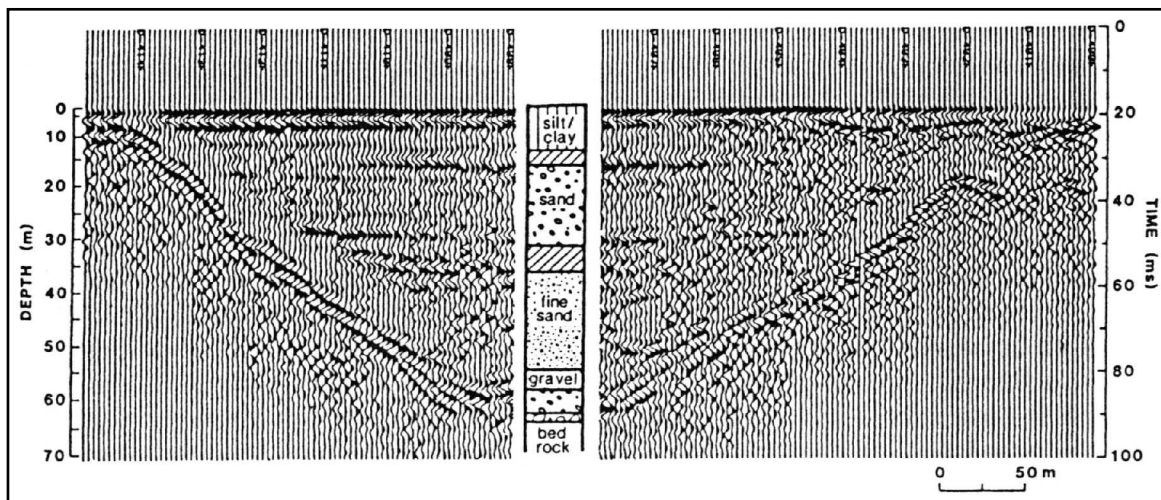
Figure 3: Seismic reflection section from Dryden, Ontario, showing a steep-sided valley in the bedrock, filled with clay and sand deposits, from Pullan and Hunter (1990), by permission. The section is approximately 500 m in length.
