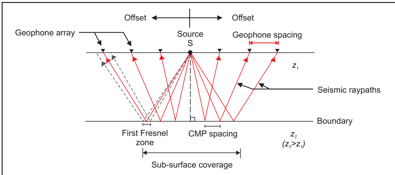
Figure 1: Schematic of reflection raypaths over a horizontal interface between materials of differing acoustic impedance ( z ), where z_2 > z_1 .
