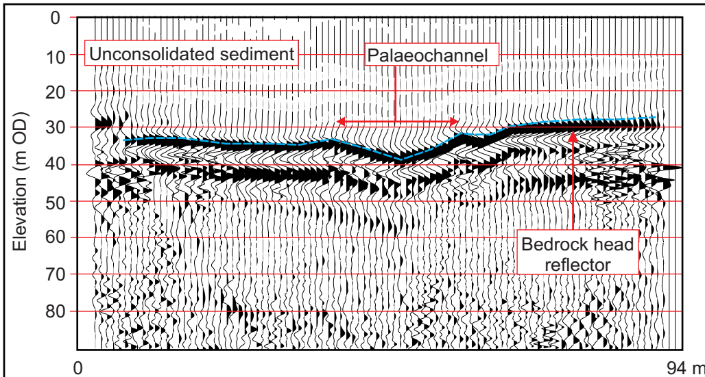
Figure 2: Seismic reflection section from a survey to detect sandstone bedrock beneath unconsolidated sediments in the Mersey Estuary, UK.
