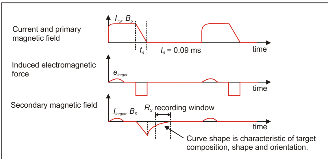
Figure 2: EM61 waveforms demonstrating relationship of primary magnetic field B_p to generation and decay of secondary magnetic field B_s . Reproduced from McNeill & Bosnar, 1996.
