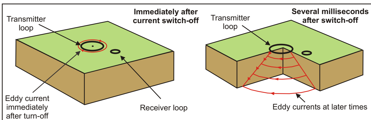
Figure 1: The measurement process for acquisition of TEM data.
