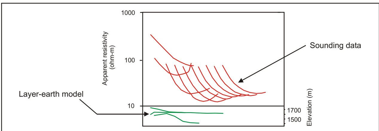
Figure 4: An interpreted layer-earth model derived from a sequence of sounding data along a single profile line, produced using TEMIX software (courtesy of Interpex Ltd).
