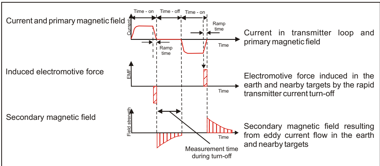
Figure 2: Time domain EM waveforms (courtesy of D. McNeill/SEG).
