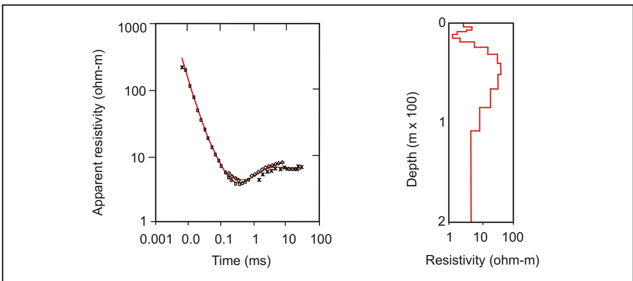
Figure 3: Right: A sounding model obtained using TEMIX software derived from the sounding curve (left). (Courtesy of Interpex Ltd).
