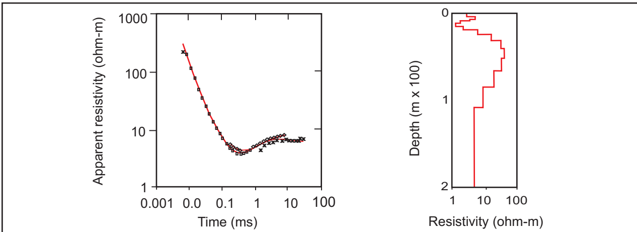
Figure 3: Right: A sounding model obtained using TEMIX software derived from the sounding curve (left). (Courtesy of Interpex Ltd).
