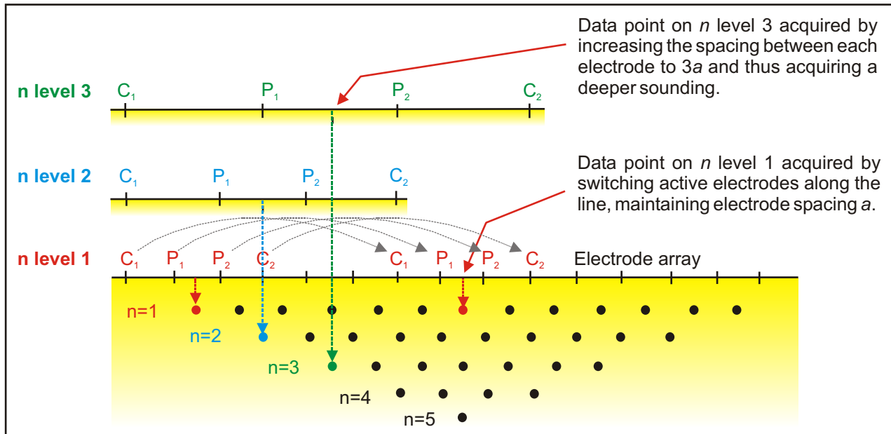
Figure 2: Example of data acquisition geometry during a 2D electrical tomographic survey, showing how increasing electrode spacing facilitates study of deeper ground materials.
